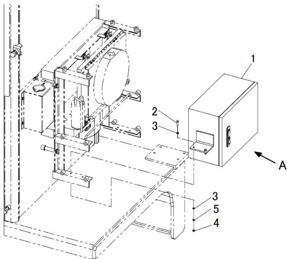
FIG.721 ELECTRICAL SYSTEM (RELAY BOX)
