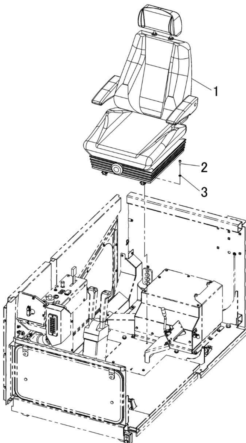
FIG.238 OPERATOR'S SEAT
