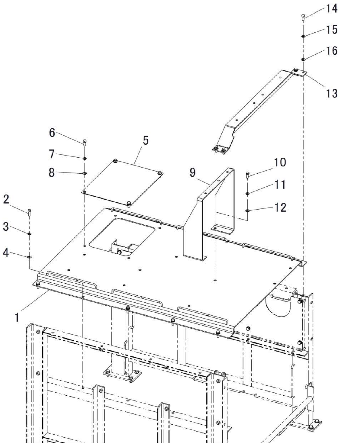
FIG.204-2 FRAME RELATED PARTS (MUFFLER BASE)
