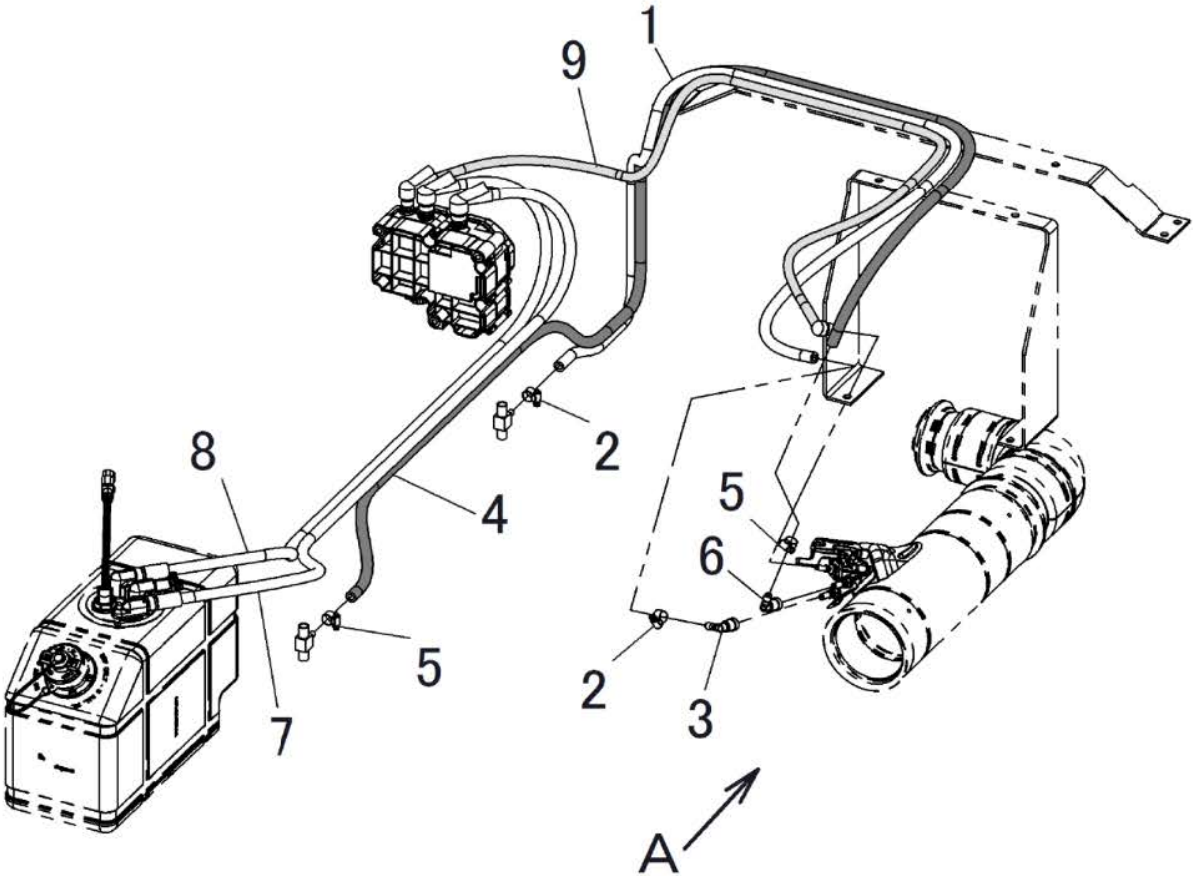
FIG.133-3 DEF PIPING (3/3)
