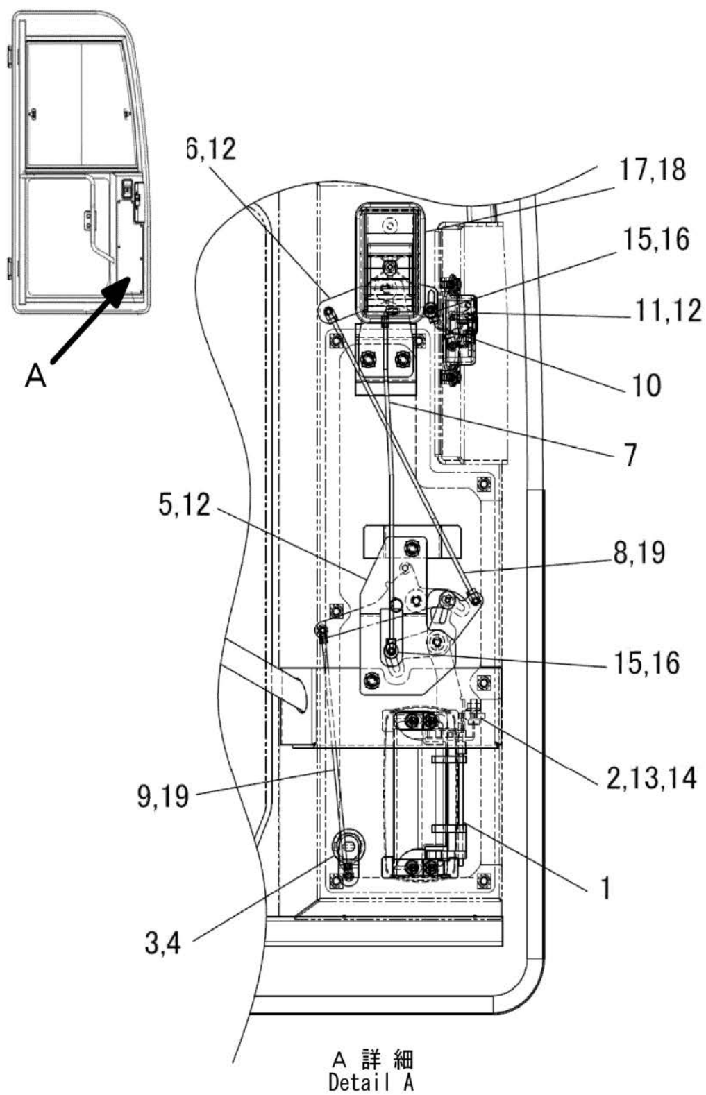
FIG.232 CAB RELATED PARTS (2/7)
