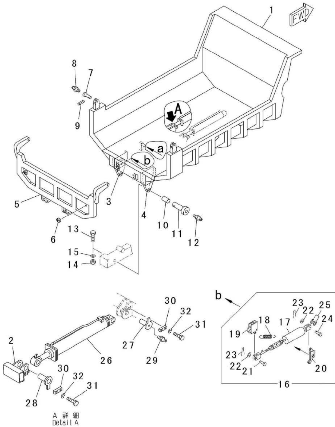
FIG.601 DUMP BODY RELATED PARTS (EARTH MOVER TYPE)
