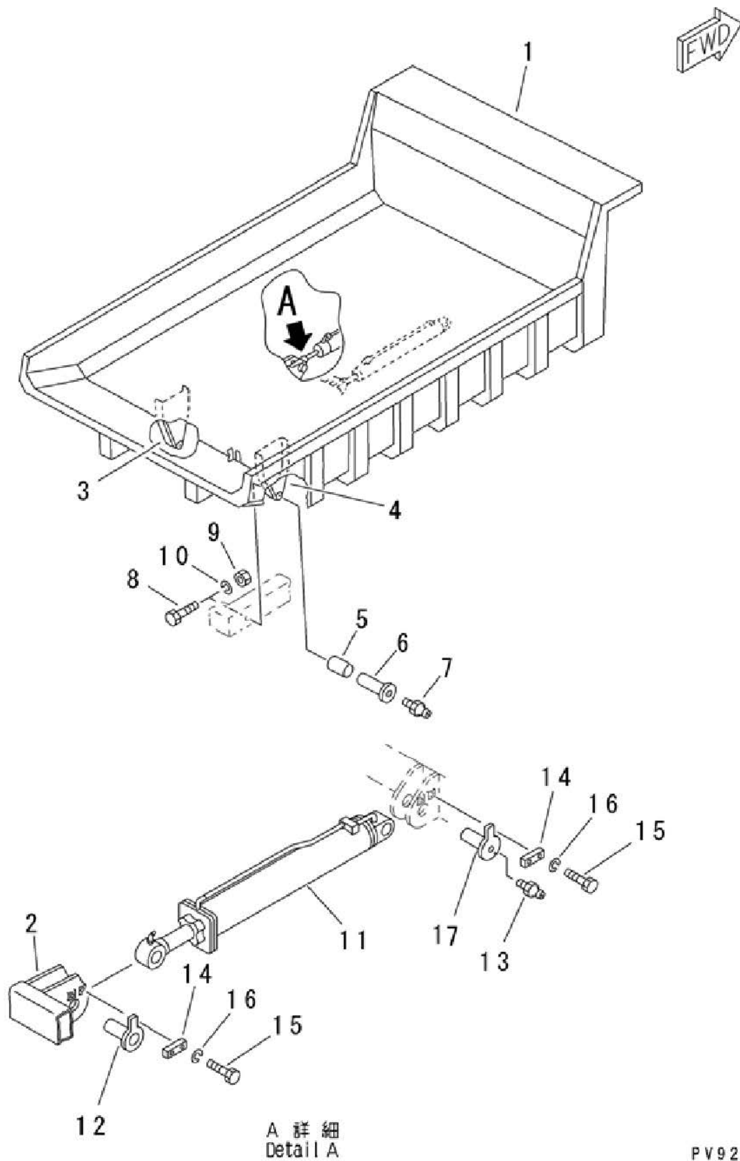
FIG.611 DUMP BODY RELATED PARTS (SCOOP END TYPE)
