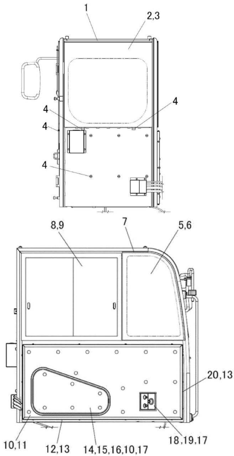
FIG.234 CAB RELATED PARTS (4/7)
