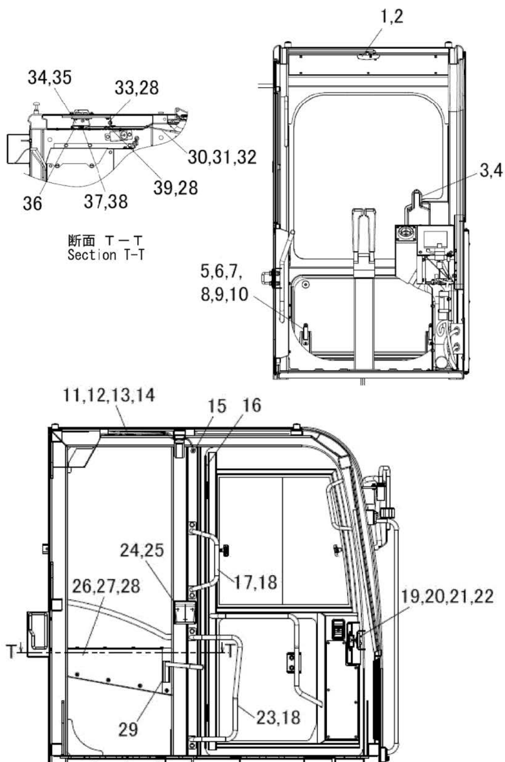
FIG.325 CAB RELATED PARTS (5/7)
