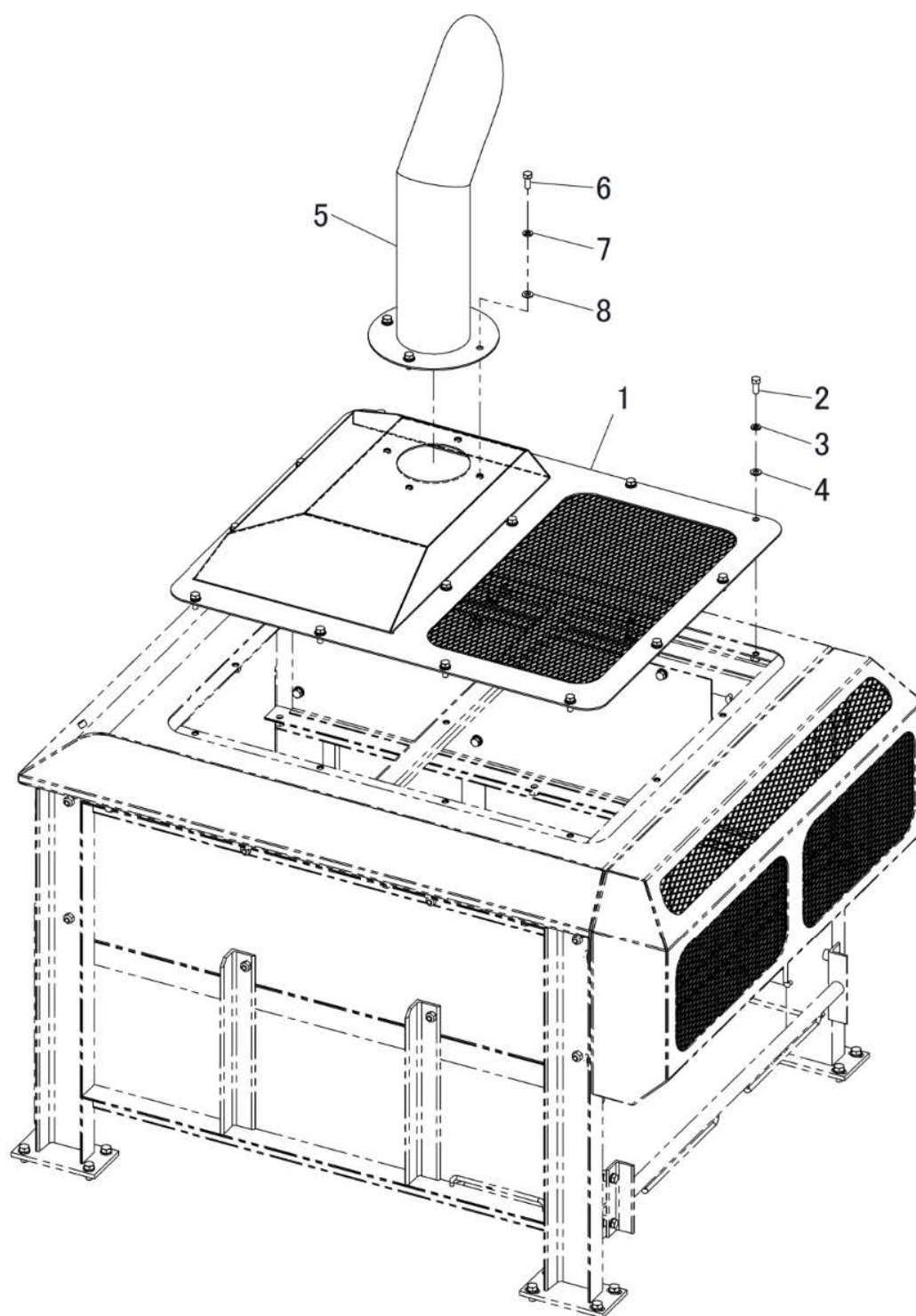
FIG.204-3 FRAME RELATED PARTS(EXHAUST PIPE)
