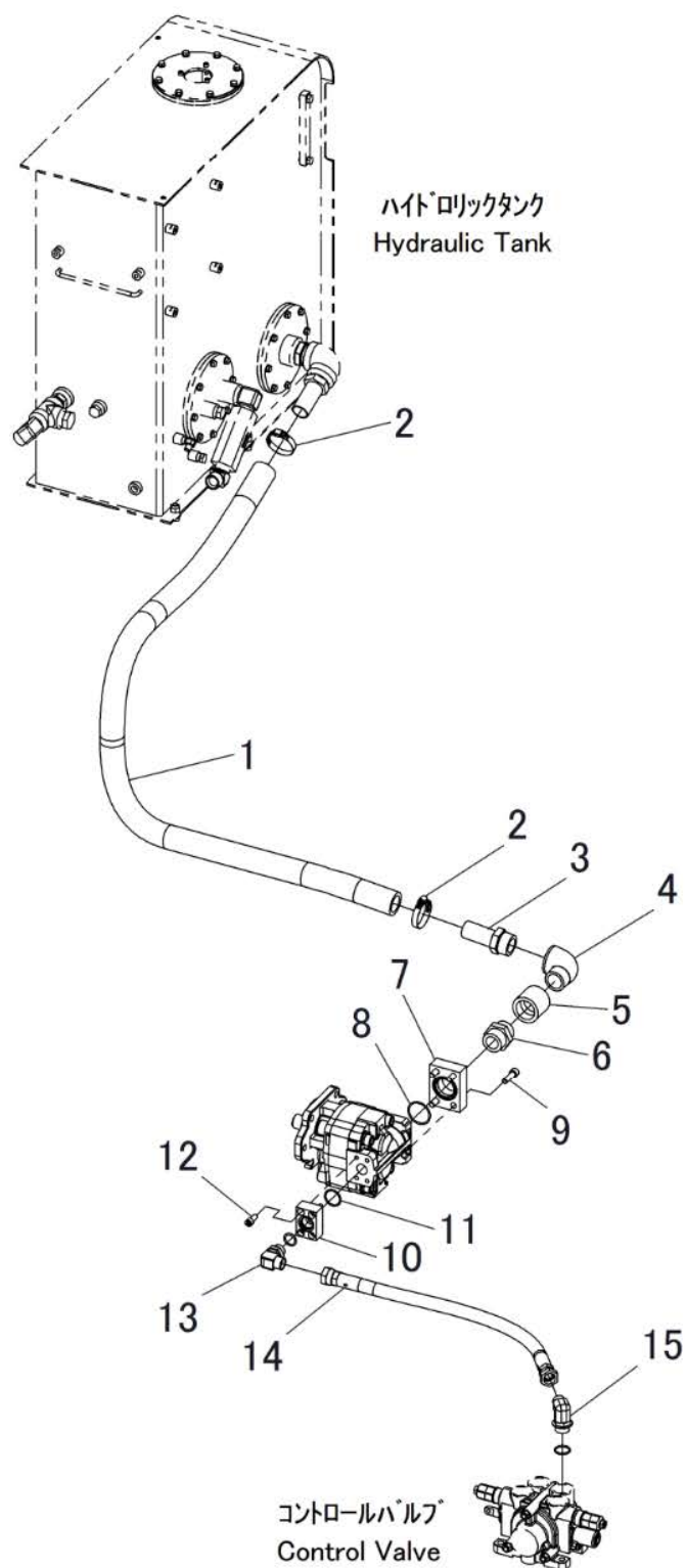
FIG.501-1 HYDRAURIC PIPING (CONTROL VALVE AND DUMP CYLINDER LINE) (1/2)
