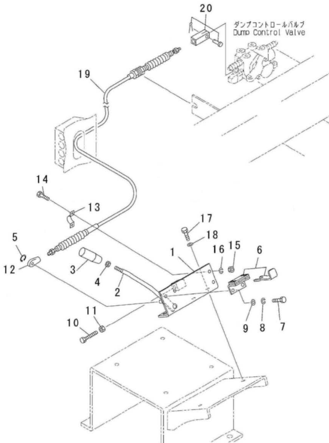
FIG.421 DUMP CONTROL SYSTEM
