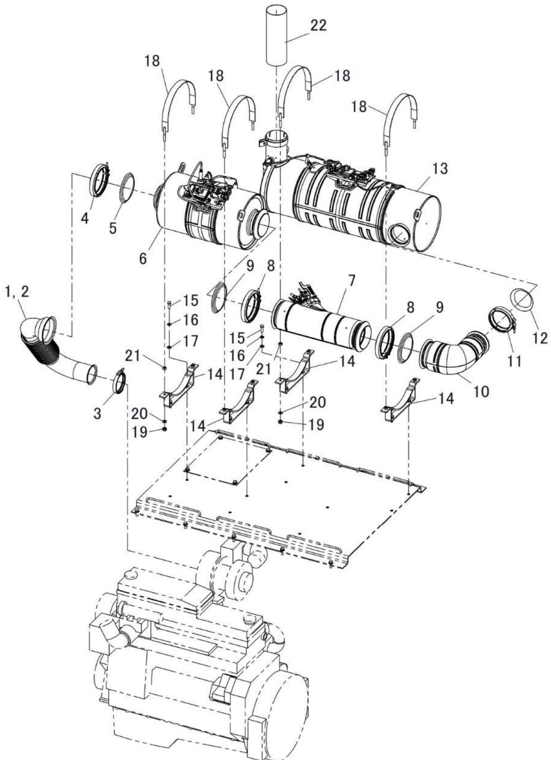
FIG.115 ENGINE RELATED PARTS (EXHAUST SYSTEM)
