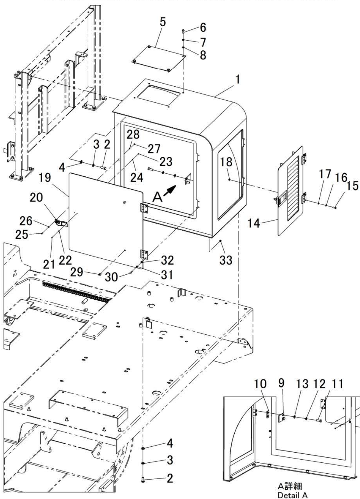
FIG.206 FRAME RELATED PARTS (AIR CLEANER COVER)
