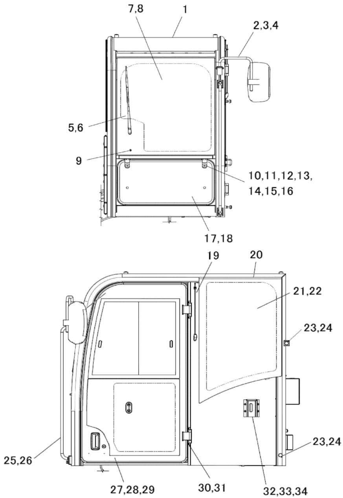
FIG.233 CAB RELATED PARTS (3/7)
