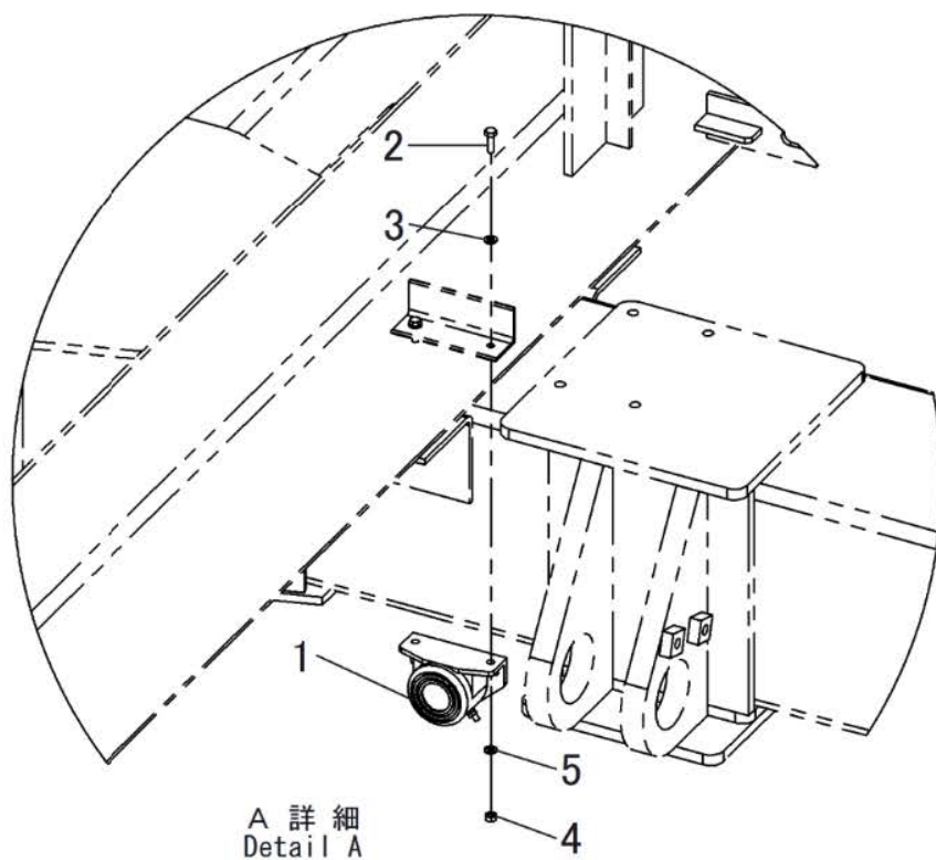
FIG.711-3 ELECTRICAL SYSTEM (BACK-UP BUZZER)
