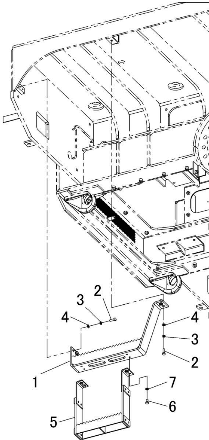
FIG.202-3 FRAME RELATED PARTS(STEP)
