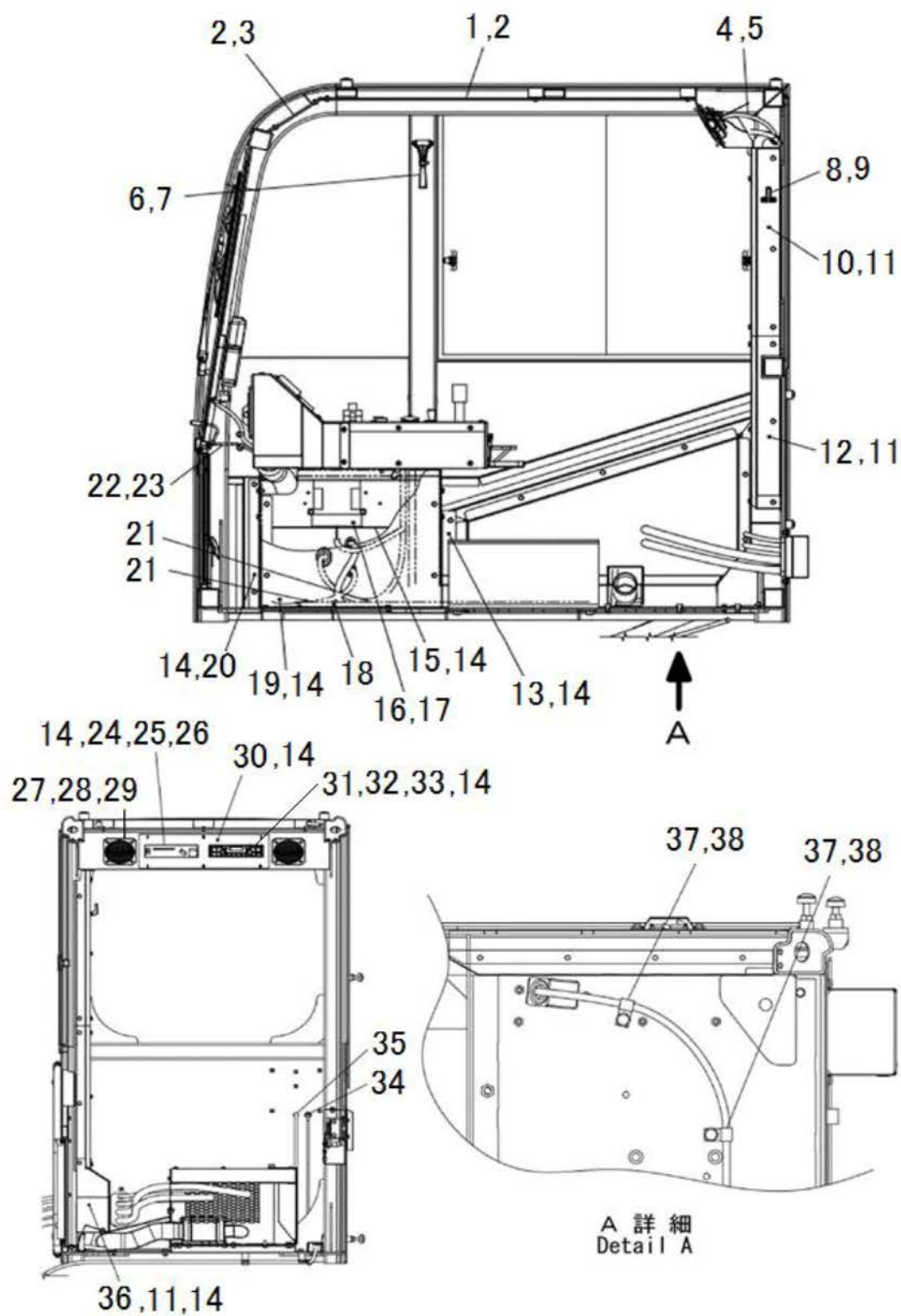
FIG.236 CAB RELATED PARTS (6/7)
