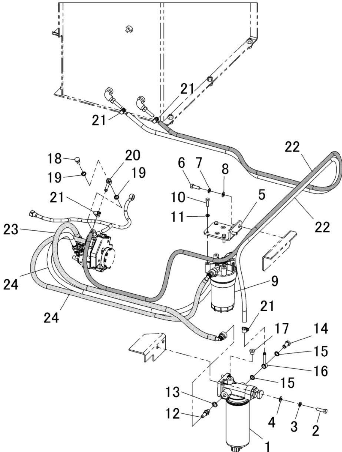
FIG.121-2 FUEL TANK AND FUEL PIPING(2/2)
