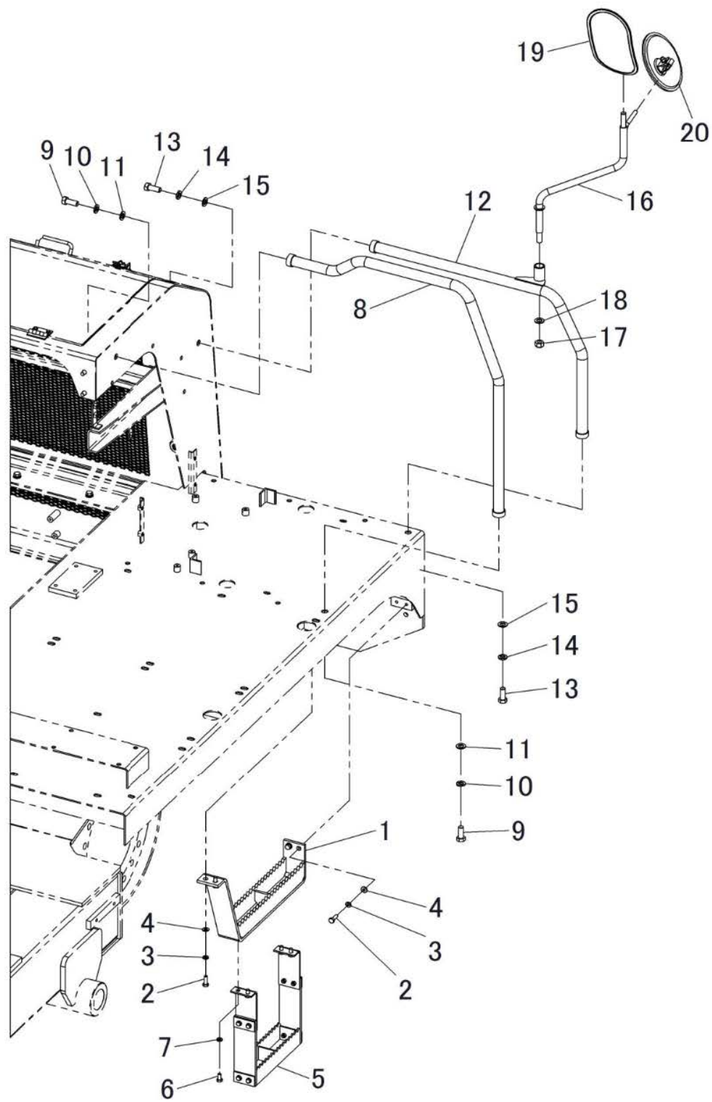
FIG.202-4 FRAME RELATED PARTS (HAND RAIL AND STEP)
