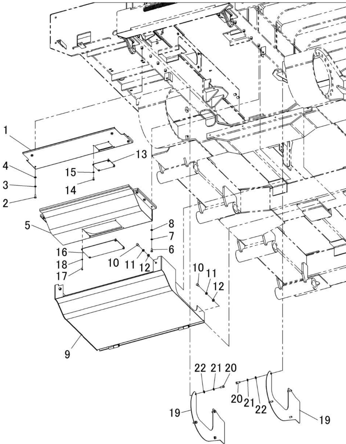
FIG.202-1 FRAME RELATED PARTS(UNDER COVER)
