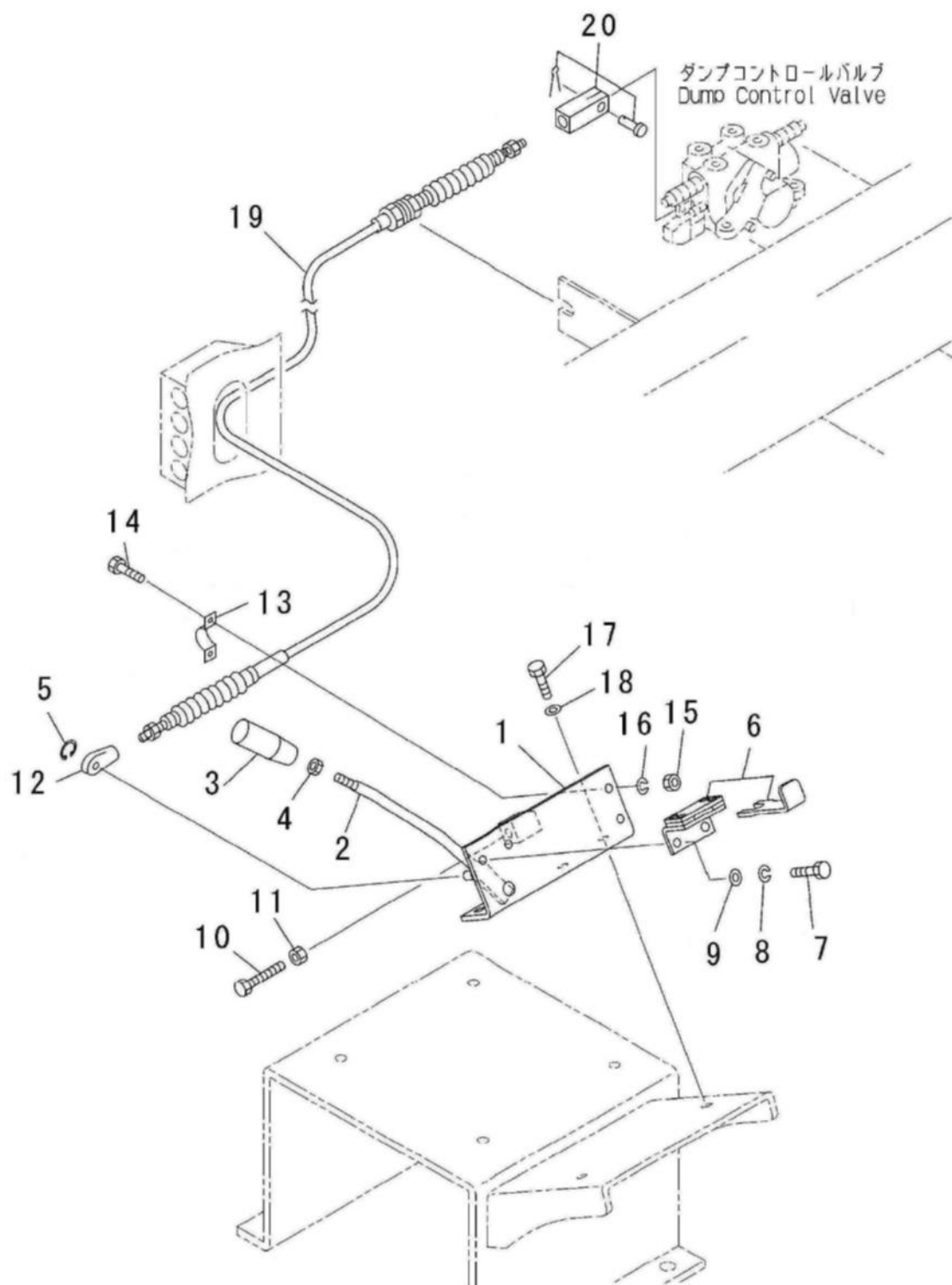
FIG.421 DUMP CONTROL SYSTEM
