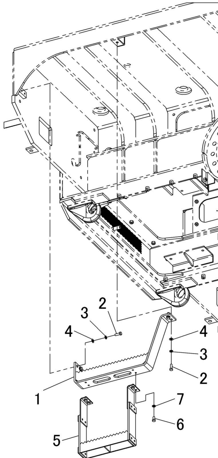
FIG.202-3 FRAME RELATED PARTS (STEP)
