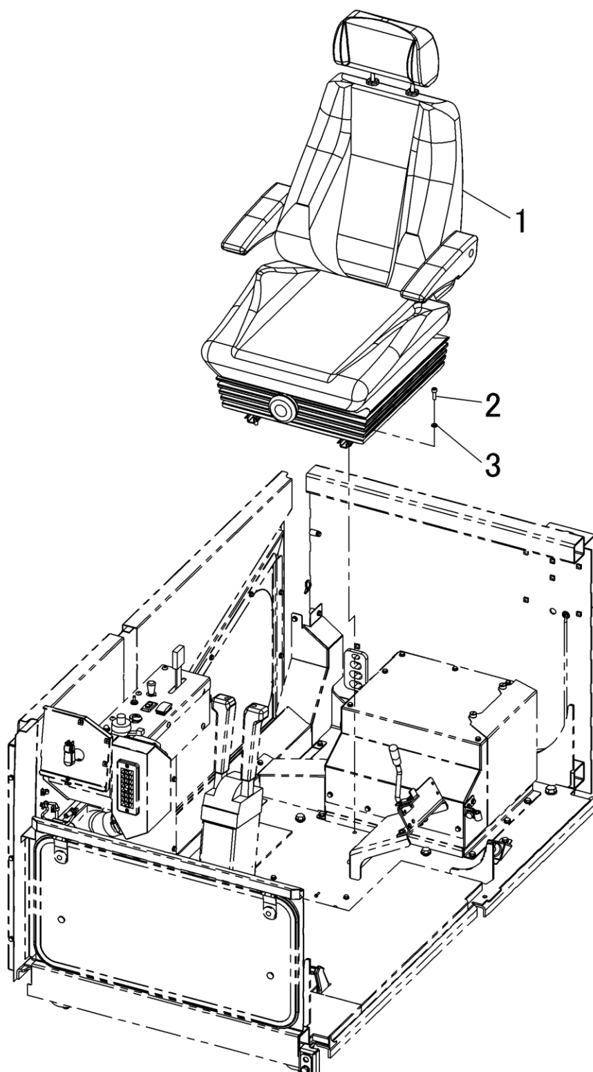
FIG.238 OPERATOR'S SEAT
