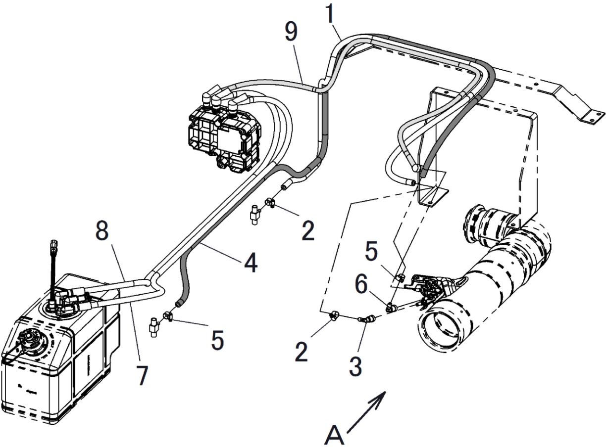
FIG.133-3 DEF PIPING (3/3)
