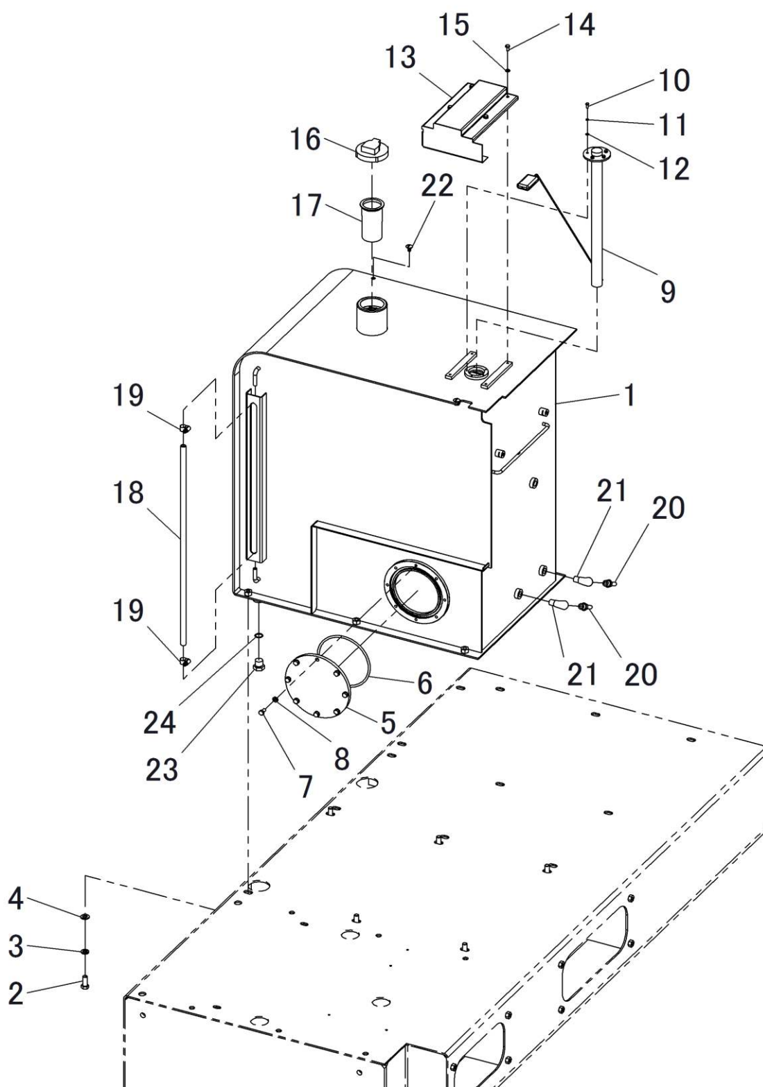
FIG.121-1 FUEL TANK AND FUEL PIPING(1/2)
