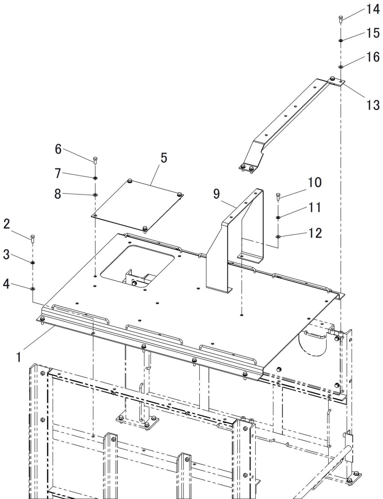
FIG.204-2 FRAME RELATED PARTS (MUFFLER BASE)
