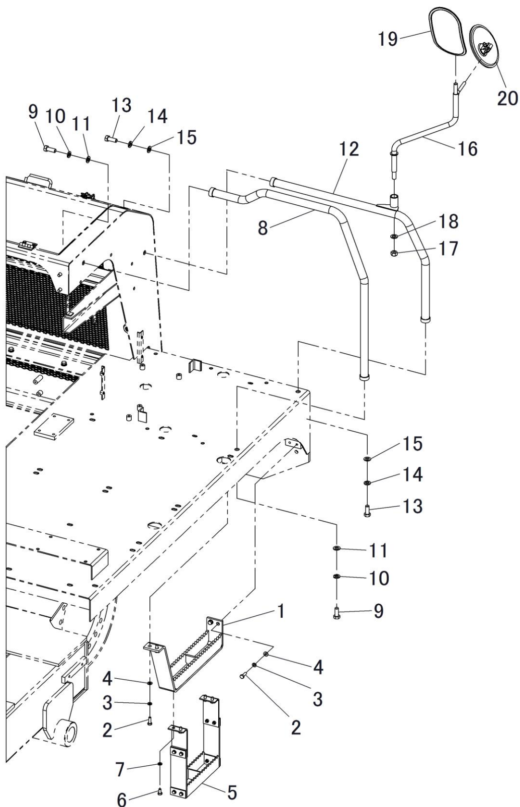
FIG.202-4 FRAME RELATED PARTS(HAND RAIL AND STEP)
