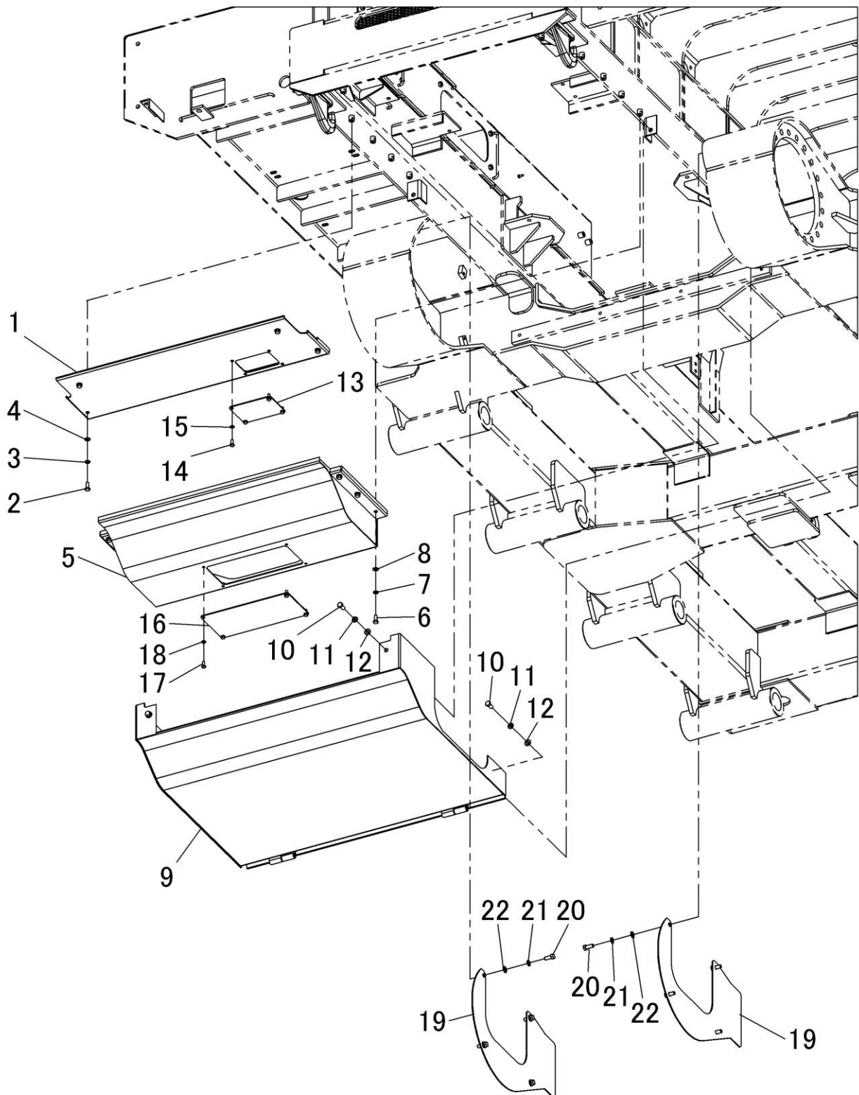
FIG.202-1 FRAME RELATED PARTS(UNDER COVER)
