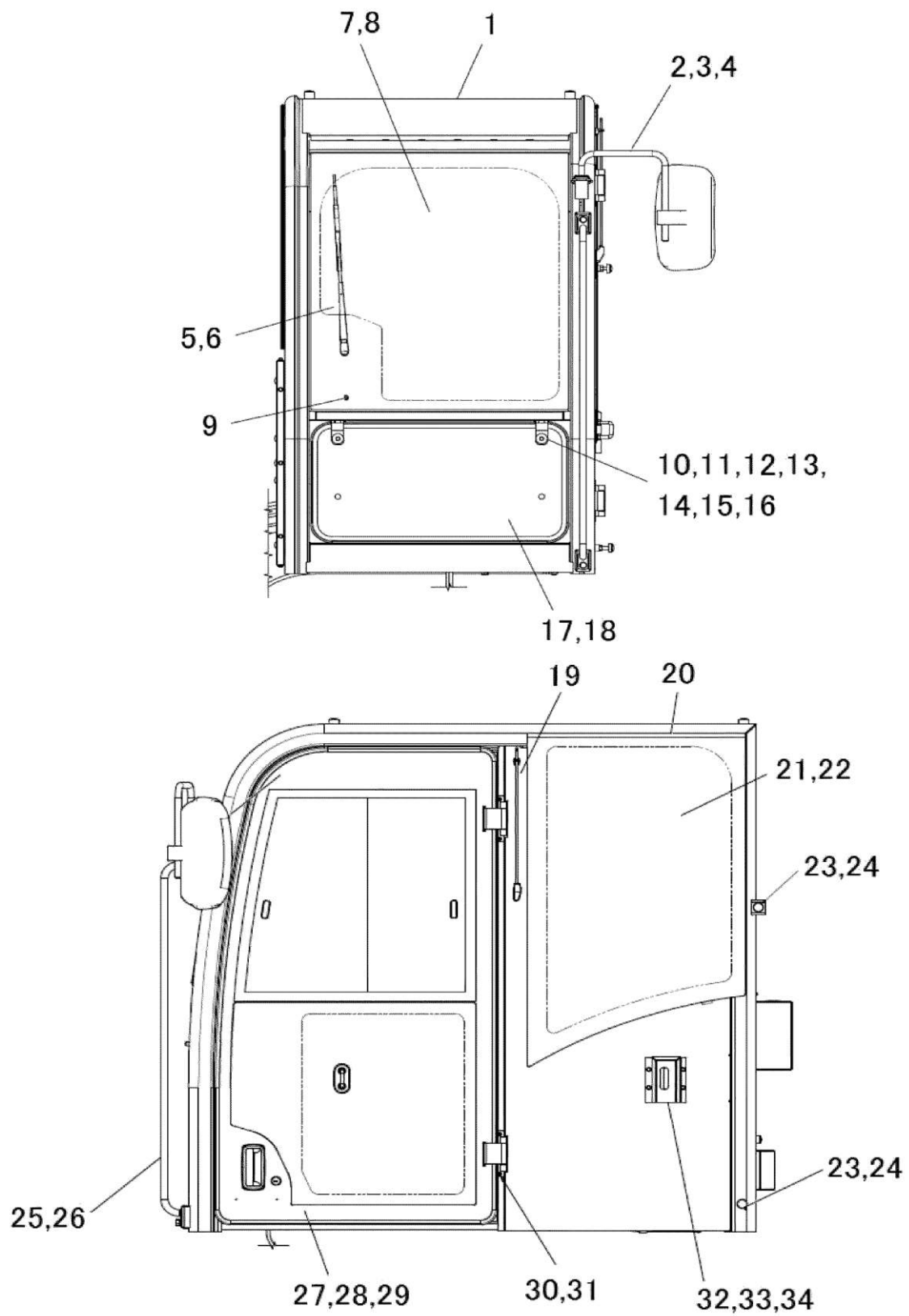
FIG.233 CAB RELATED PARTS (3/7)
