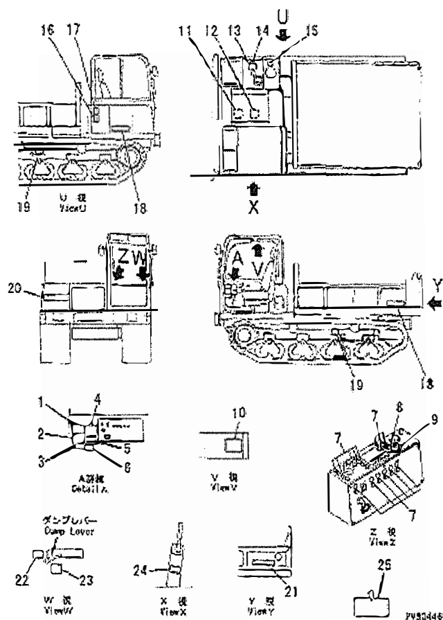
FIG.811 MARKS AND CAUTION PLATES (ENGLISH) (APPLICABLE TO CAB SPEC.)
