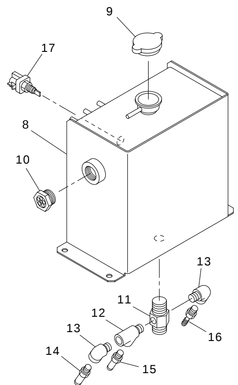
"B" DETAIL
