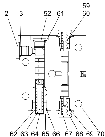
"C-C" SECTION
