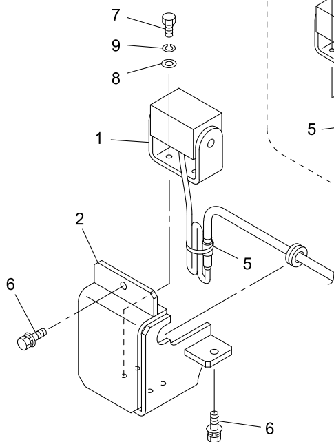
"B" DETAIL
