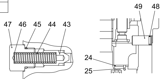
"D-D" SECTION
