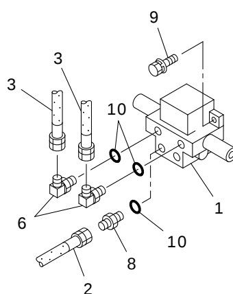
"B" DETAIL
