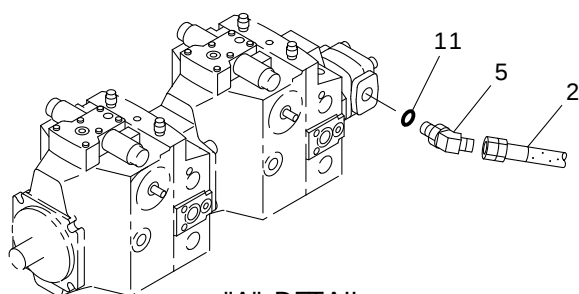
"A" DETAIL
