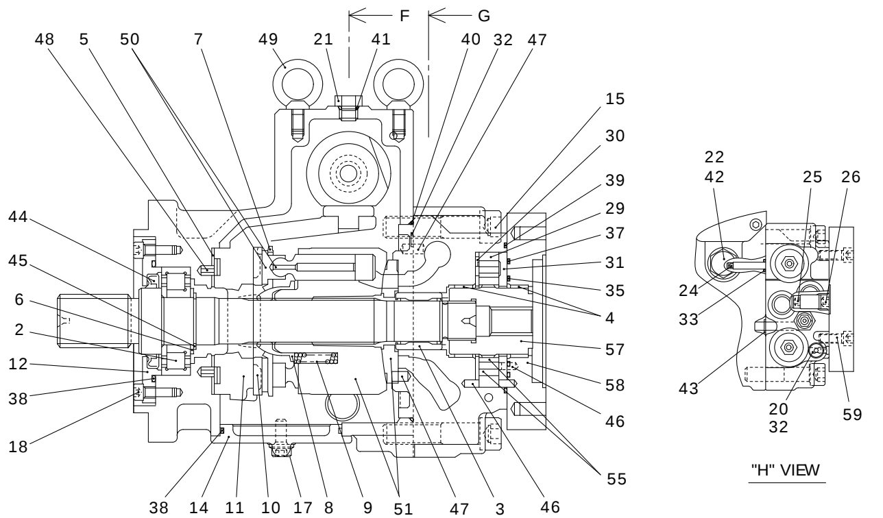
"B" DETAIL
