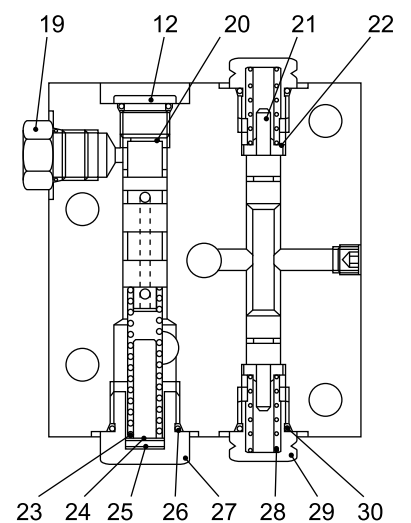
"C-C" SECTION
