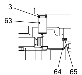
"E-E" SECTION
