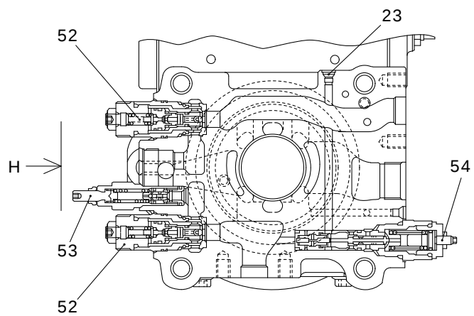
"G- G" SECTION
