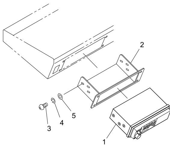
"A" VIEW
