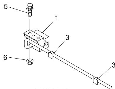
"B" DETAIL
