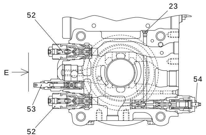
"D- D" SECTION
