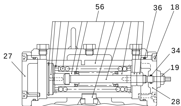
"C- C" SECTION
