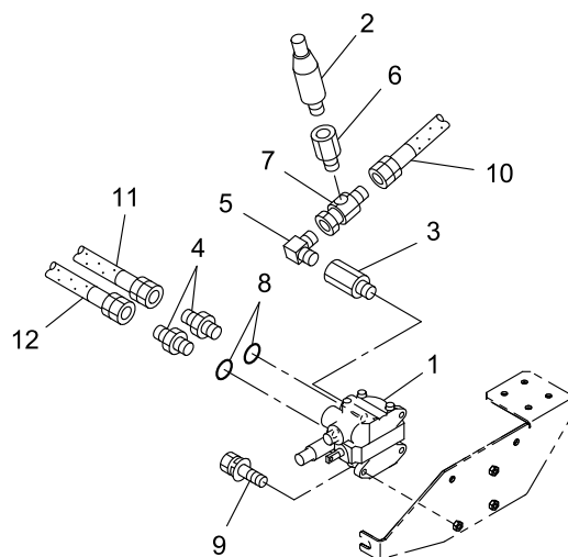
C DETAIL
