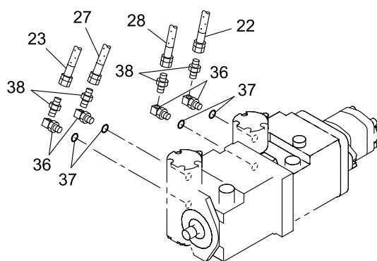
B DETAIL
