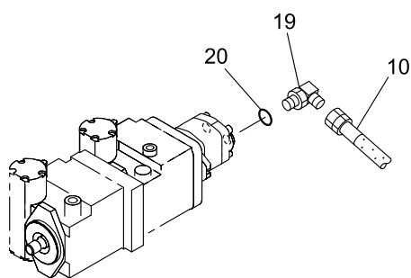
A DETAIL
