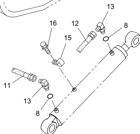
D DETAIL
