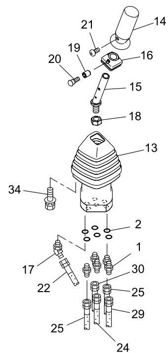
A DETAIL
