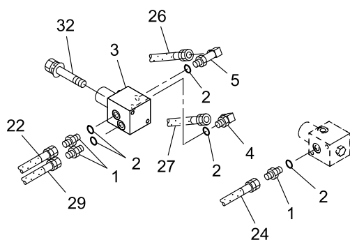
D DETAIL
