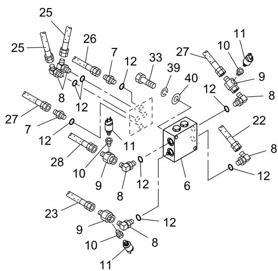
E DETAIL
