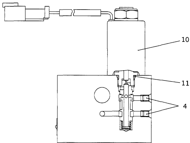
"C-C" SECTION
