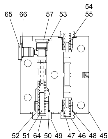
"C-C" SECTION
