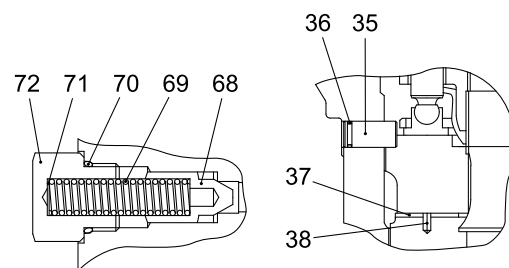
"D-D" SECTION
