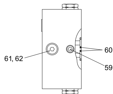
"A" DETAIL
