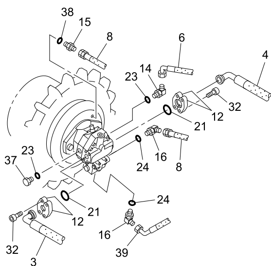
A DETAIL
