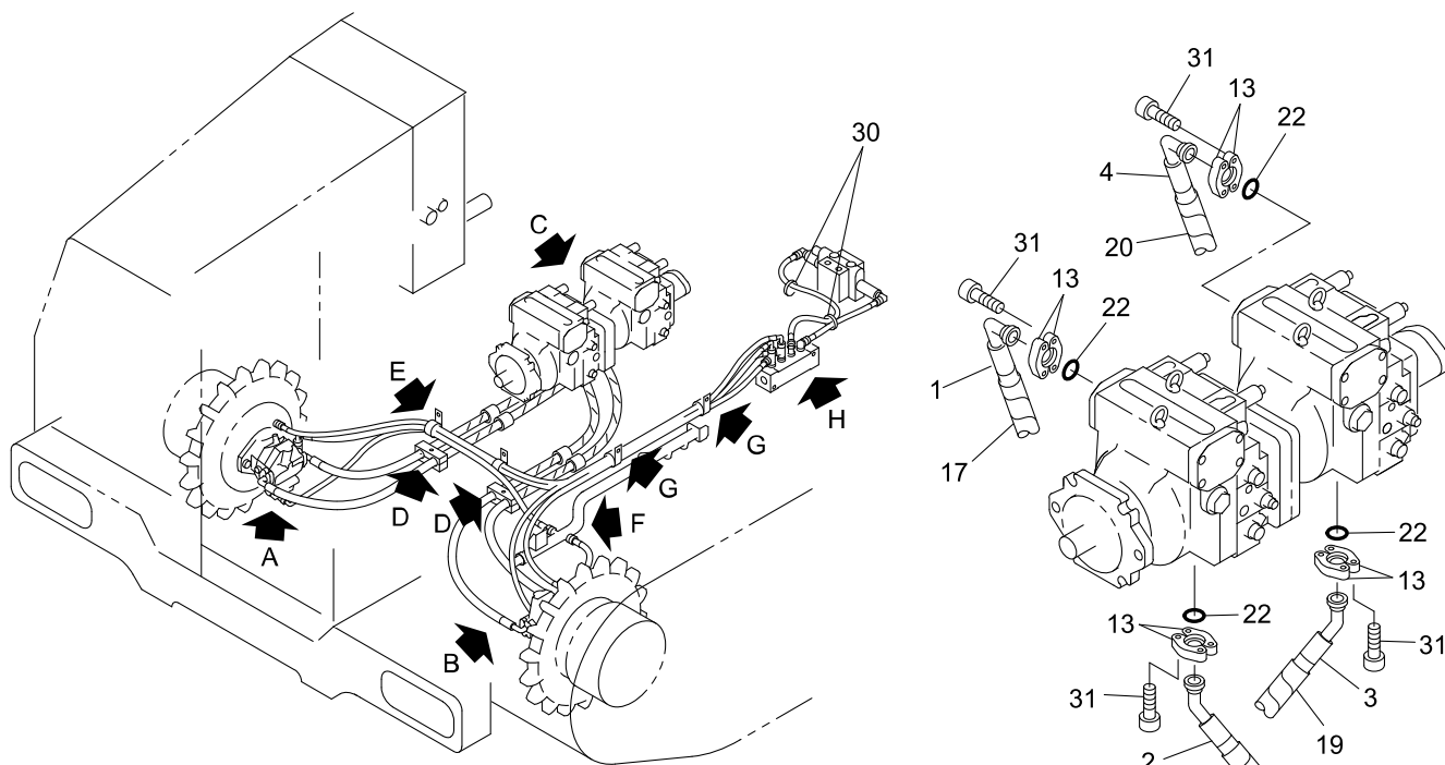
C DETAIL
