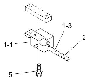
B DETAIL
