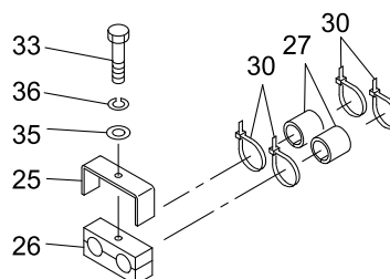
D DETAIL
