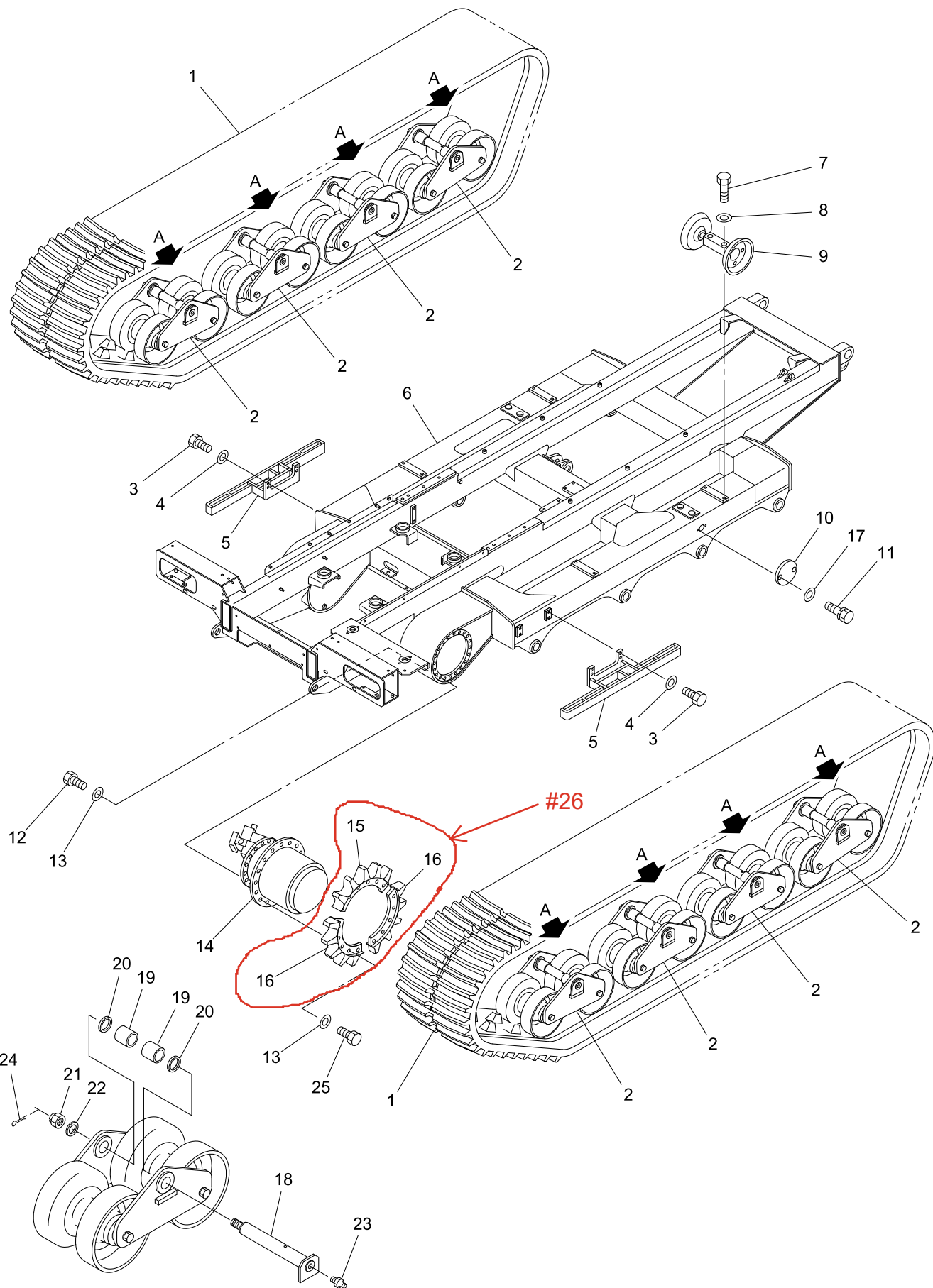
A DETAIL
