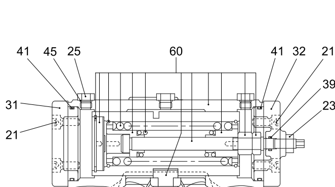
SECTION C-C
