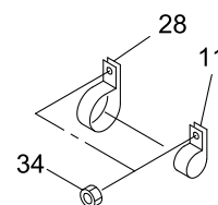
E DETAIL
