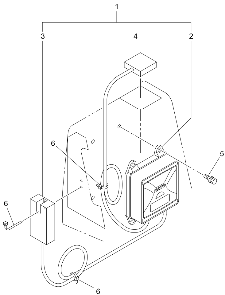
VIEW A
