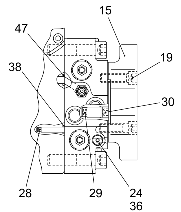
VIEW F-F
