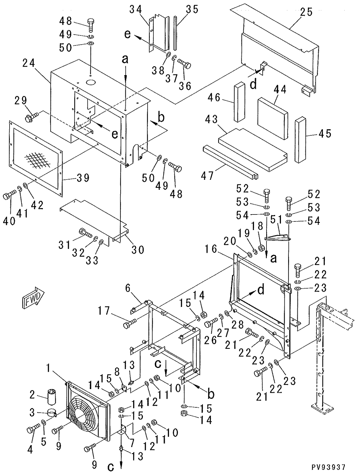
FIG. 262 AIR CONDITONER RELATED PARTS (A/C CONDENSOR AND MOUTING) (SERIAL NO.224001-224031, 224036-224041, 224043-224047, 224052)
