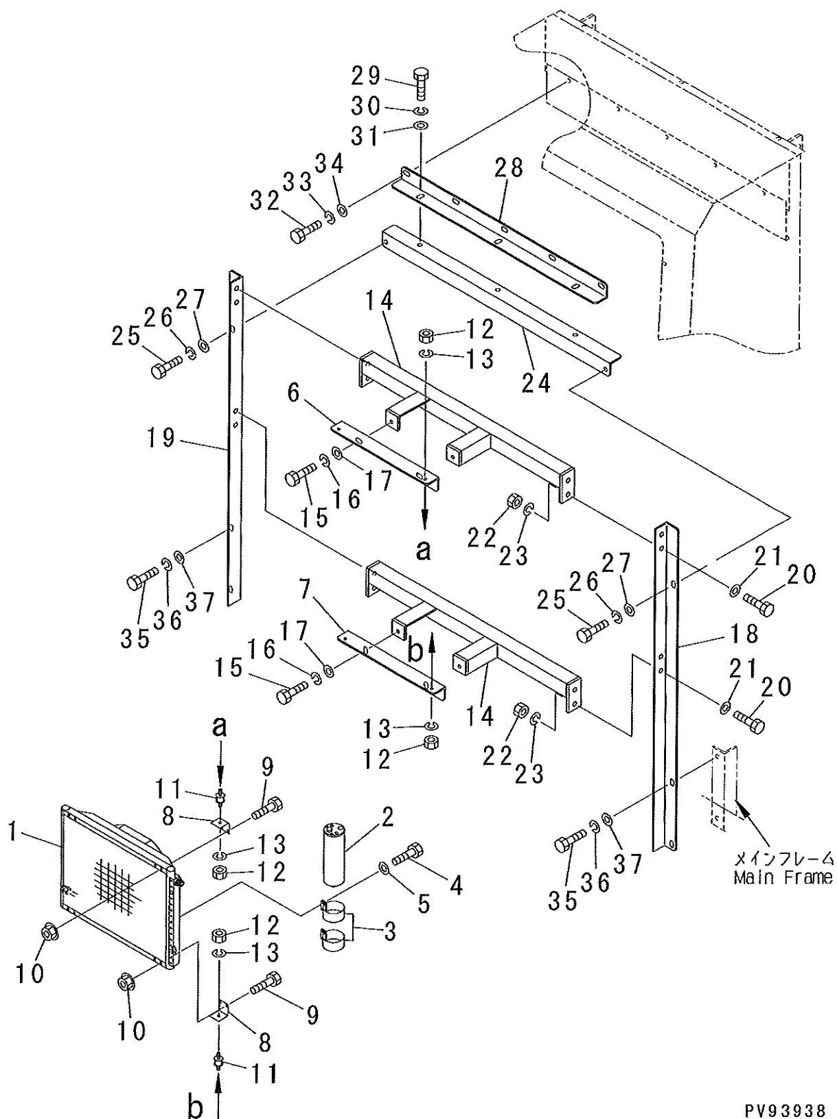
FIG. 262A AIR CONDITONER RELATED PARTS (A/C CONDENSOR AND MOUTING) (SERIAL NO.224032-224035, 224042, 224048-224051, 224053-)
