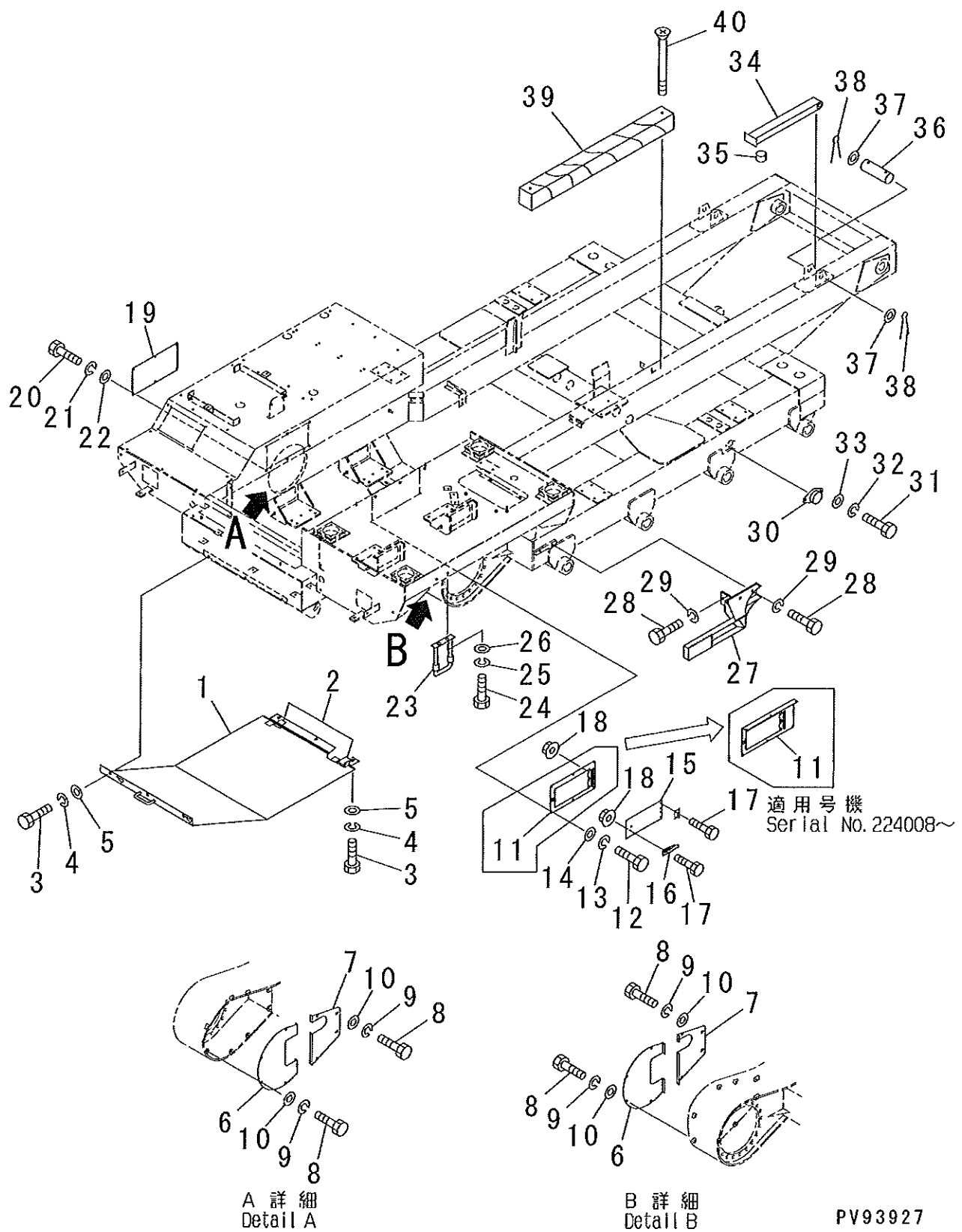
FIG. 202 FRAME RELATED PARTS (2/5) (UNDER COVER AND STEP) (SERIAL NO.224001-224017)
