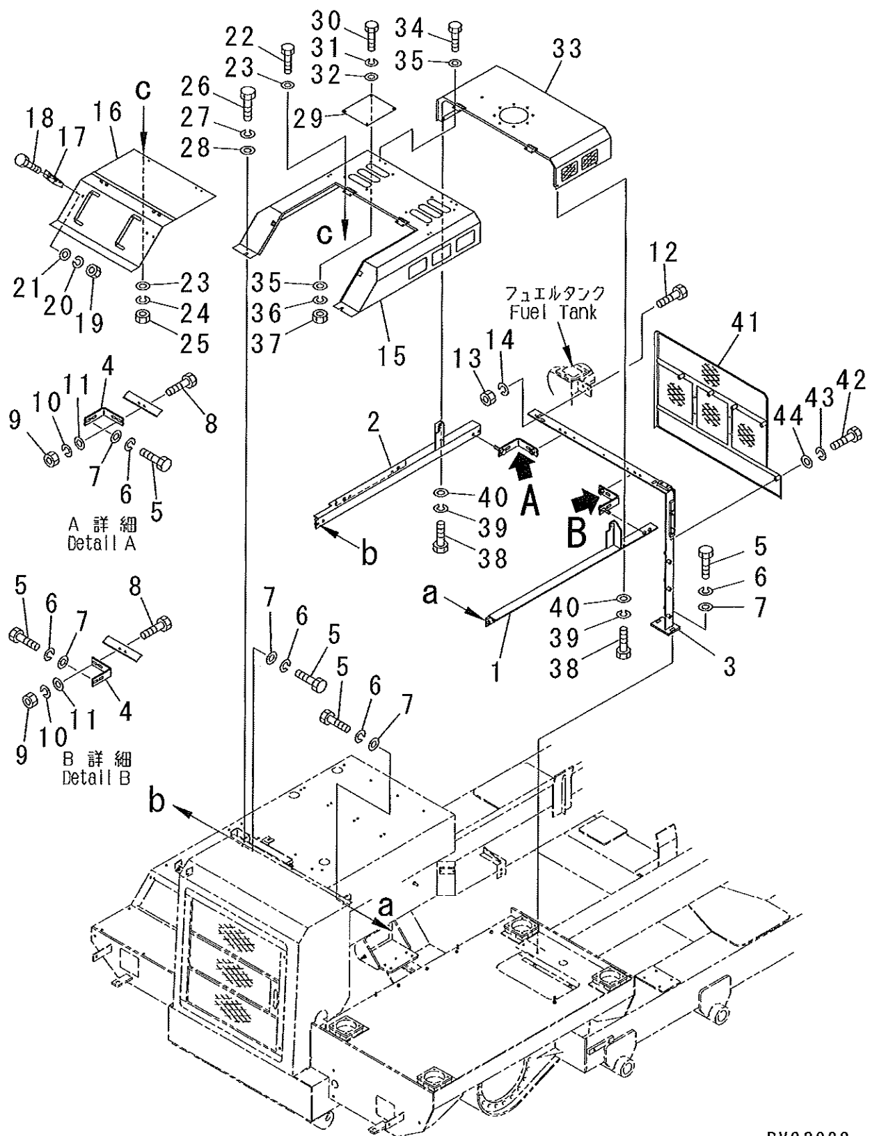
FIG. 203 FRAME RELATED PARTS (3/5) (ENGINE BONNET) (SERIAL NO.224001-224206)
