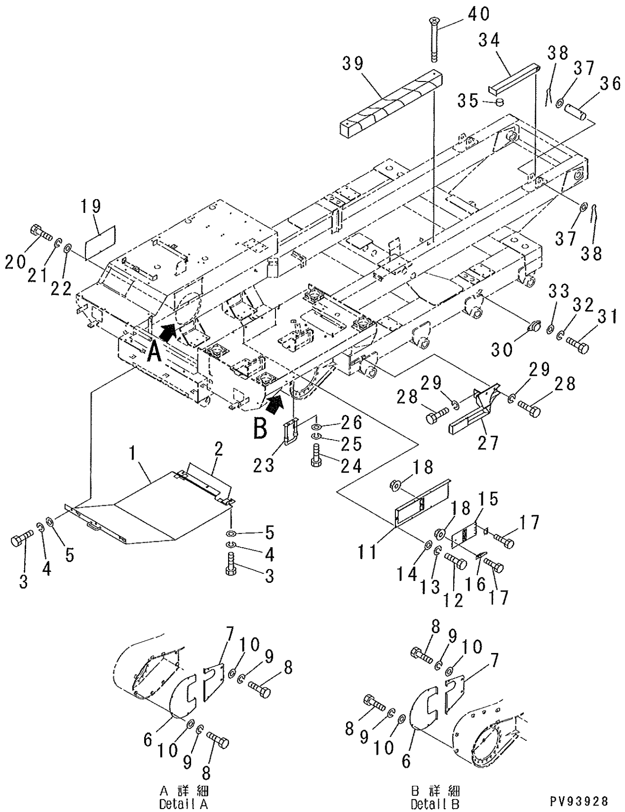
FIG. 202A FRAME RELATED PARTS (2/5) (UNDER COVER AND STEP) (SERIAL NO.224018-)
